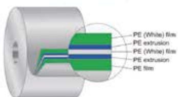
PBL tube(plastic barrier)
