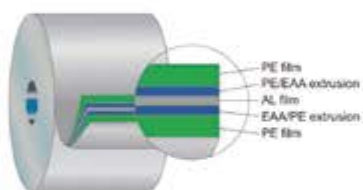
ABL tube(aluminum barrier)
